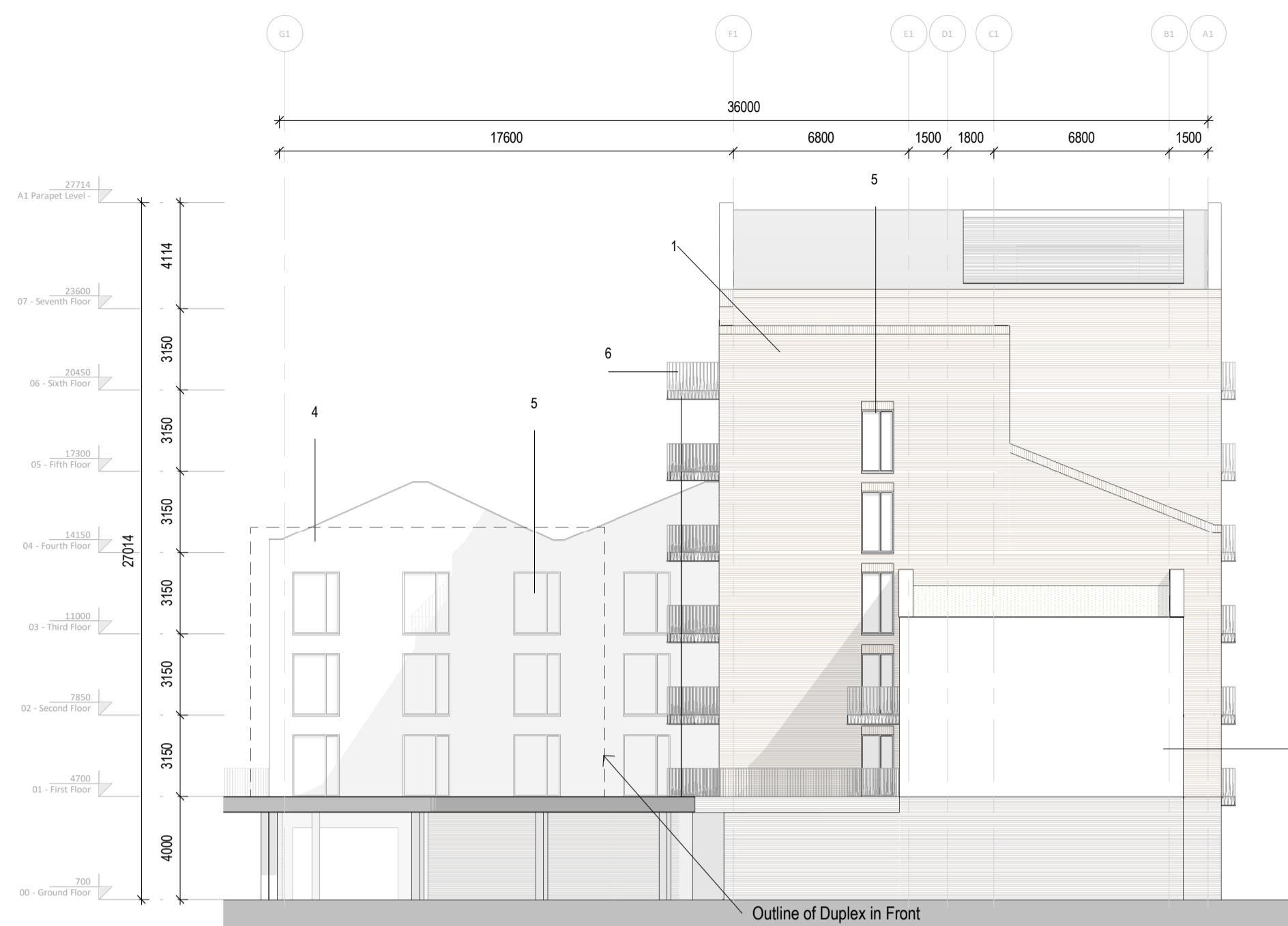
1 A1_North-East Elevation 1:200
